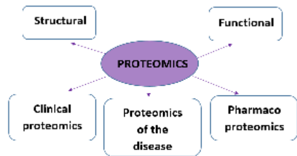
Figure 4 Current proteomics
