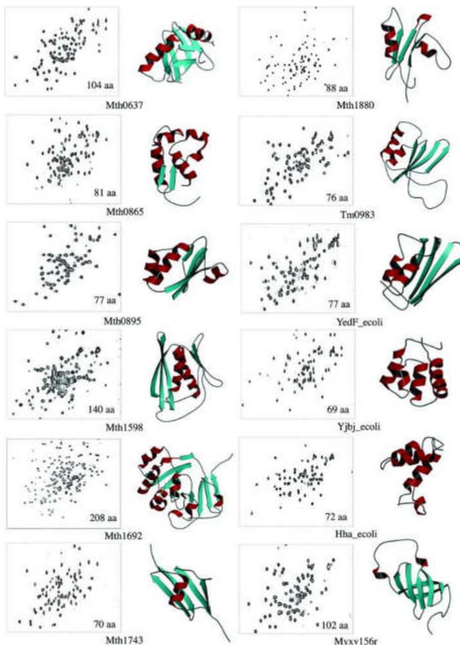
Figure 2 Protein structures [2,3]
