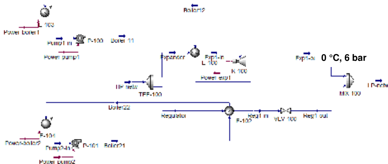
Figure 3 Aspen HYSYS model for a gas transfer station equipped with a turbo expander (upper) and a pressure regulator (lower)
